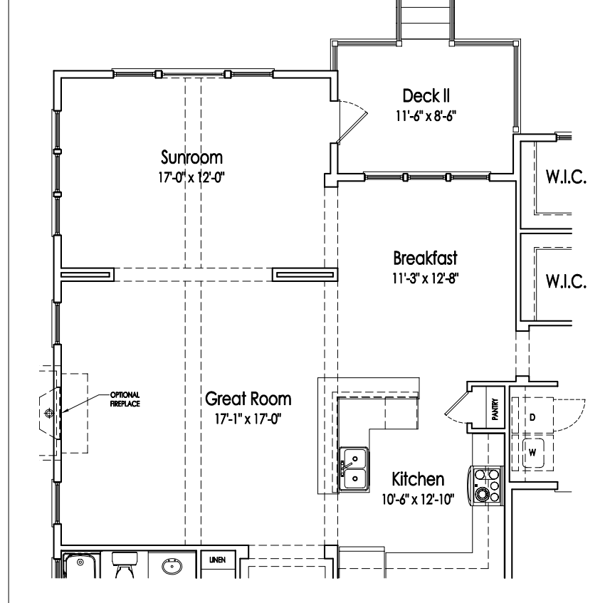
OPTIONAL SUNROOM W/ DECK II
